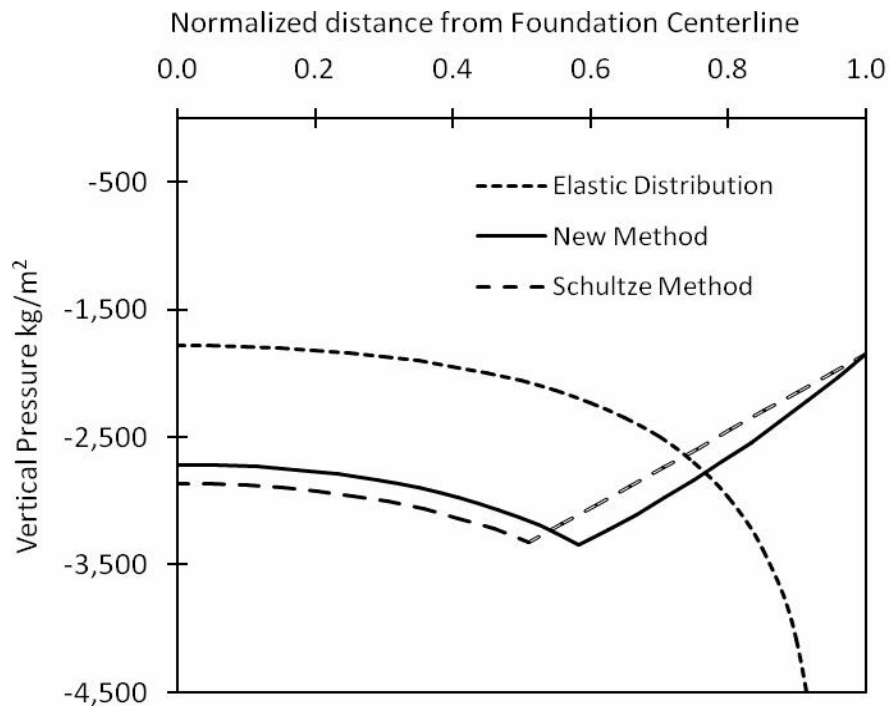
Fig. (9): Contact pressure distribution of rigid foundation on c - \phi soil, c = 24.5 \text{ kN/m}^2 , \phi = 40^\circ , \gamma = 17.3 \text{ kN/m}^3 , B = 1.2 \text{ m} , load level = 83.3%.
