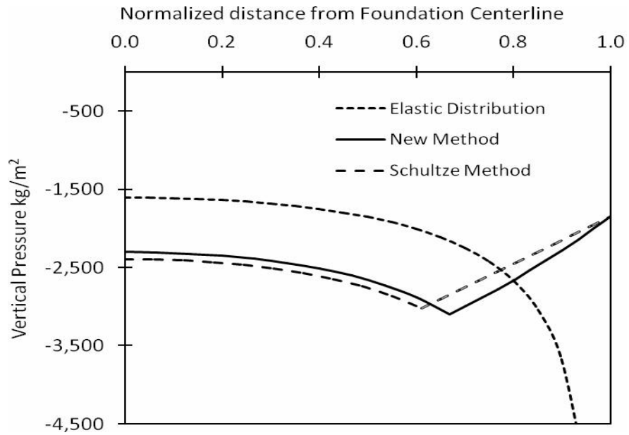
Fig. (8): Contact pressure distribution of rigid foundation on c-\phi soil, c = 24.5 \text{ kN/m}^2 , \phi = 40^\circ , \gamma = 17.3 \text{ kN/m}^3 , B = 1.2 \text{ m} , load level = 75%.
