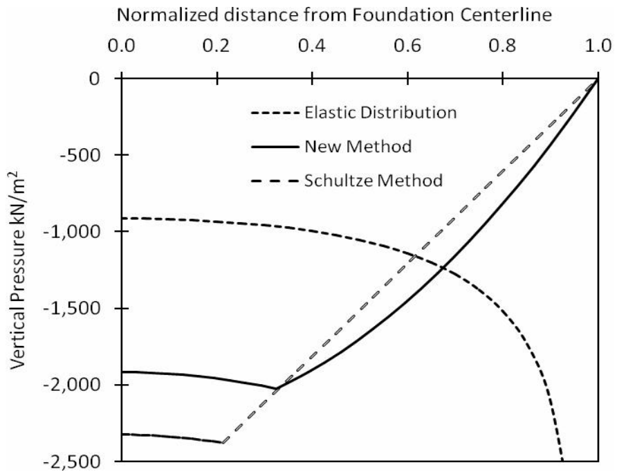
Fig. (7): Contact pressure distribution under rigid foundation on sandy soil, B = 1.2 \text{ m} , \phi = 40^\circ , \gamma = 17.3 \text{ kN/m}^3 , load level = 95%.
