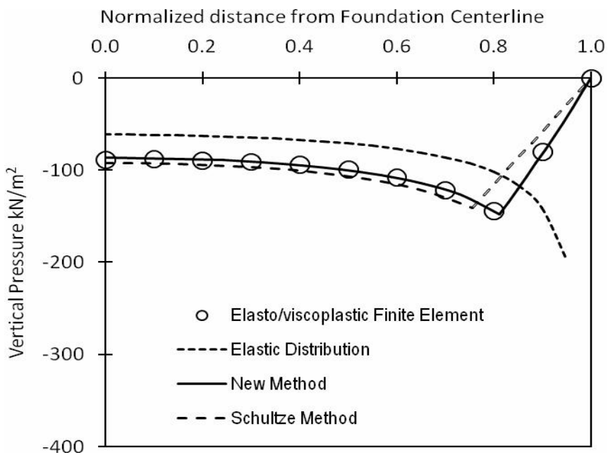
Fig. (13): Contact pressure distribution under rigid foundation on sandy soil, B = 1.524 \text{ m} , \phi = 40^\circ , \gamma = 17.3 \text{ kN/m}^3 , load level = 33.3%.
