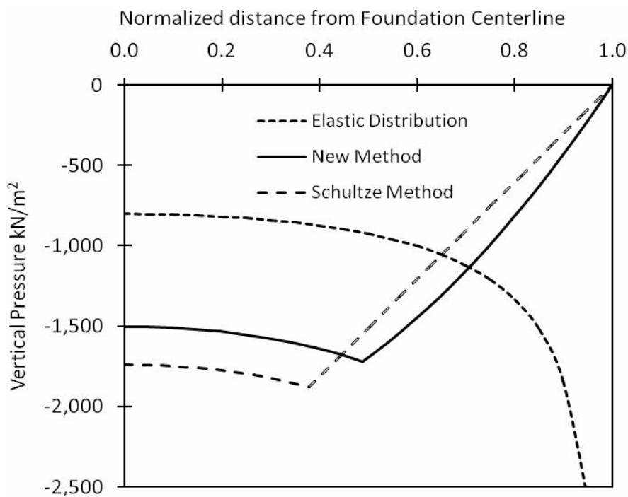
Fig. (6): Contact pressure distribution under rigid foundation on sandy soil, B = 1.2 m, \phi = 40^\circ , \gamma = 17.3 kN/m 3 , load level = 83%.
