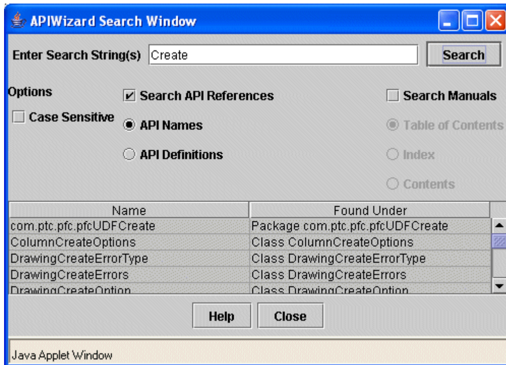
Figure 5-5: APIWizard Search Dialog Box
