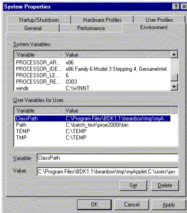
Figure 5-1: Windows NT Environment Variable Display Window
