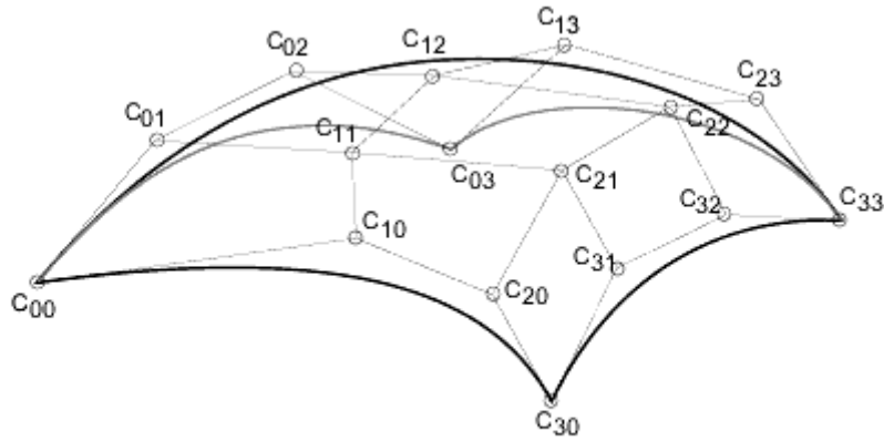
Cubic NURBS Surface
