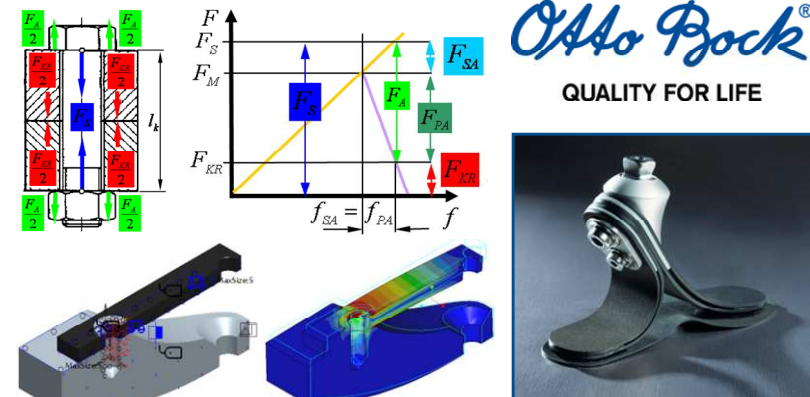
Right: The functional element of the Otto Bock 1C30 Trias prosthetic foot with carbon leaf springs and bolted connections containing typical simulation tasks treated in the advanced workshop
