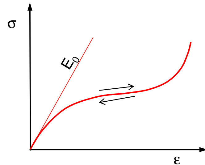
Hyperelastic material behavior
